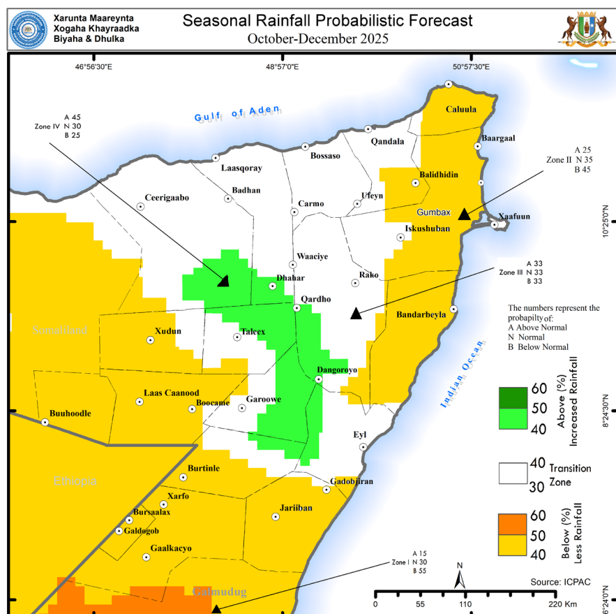
Map 1: Oct-Dec 2025 Deyr rainfall forecast
